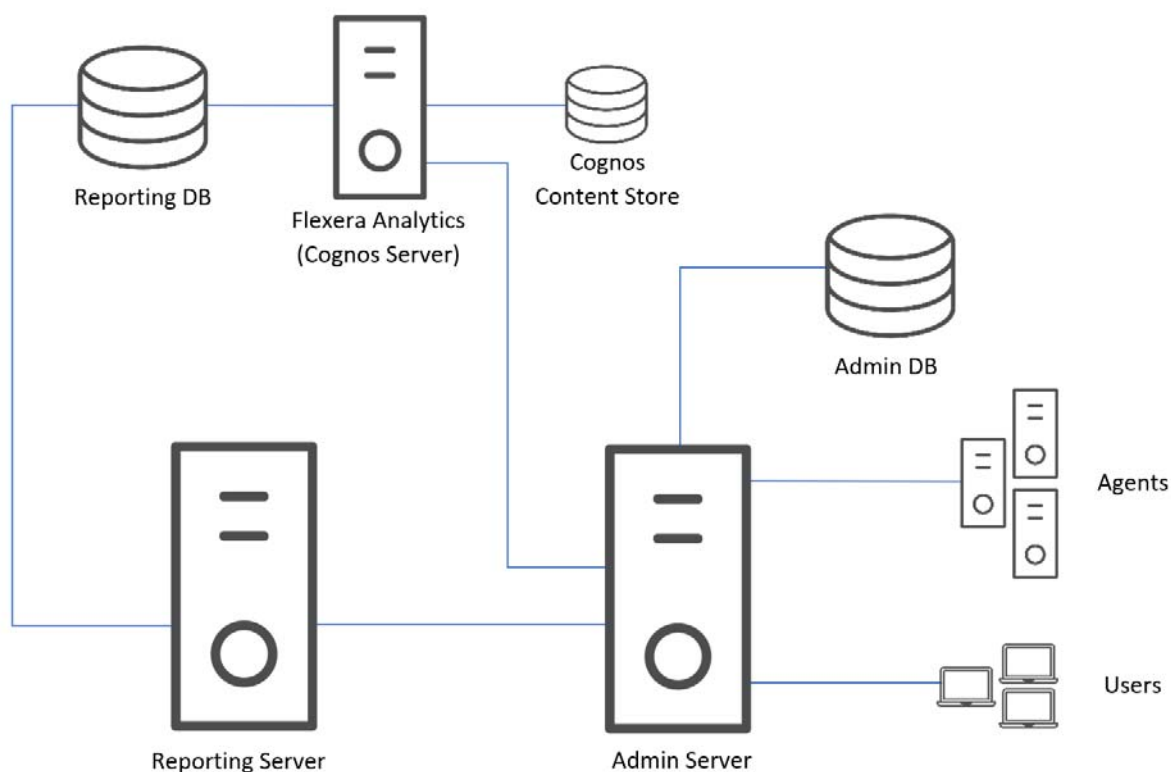
Figure 2-1: Basic FlexNet Manager for Engineering Applications deployment with Flexera Analytics (Cognos)
